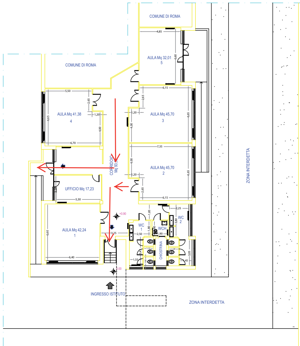
PLANIMETRIA POST-OPERAM RAPP. 1:100
